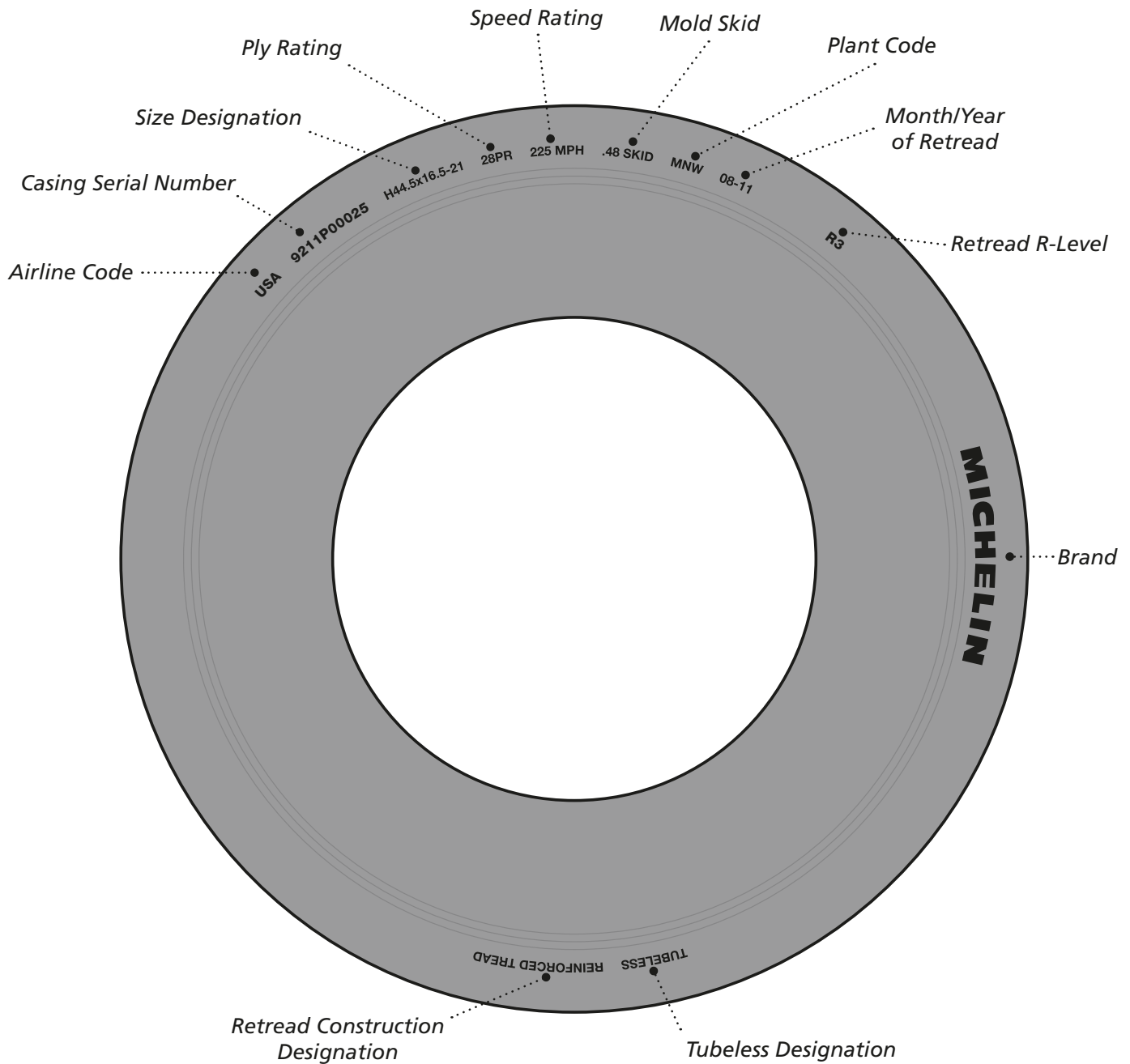
Figure 206. Typical Retread Aircraft Tire Markings
