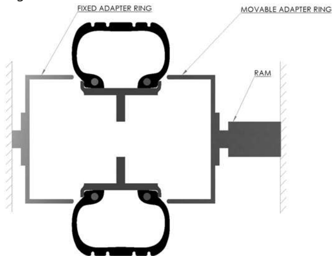
Figure 603. Ring-Type Bead Breaker
