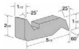
12-01281 3 Lbs.
