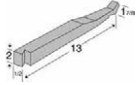
12-01301 3-1/4 Lbs.
